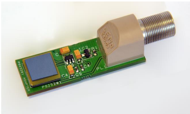
Figure 1: PS25012A single channel board carrying a single PS25201 sensor
