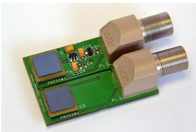
Figure 2: PS25012B dual channel board carrying two PS25201 sensors
